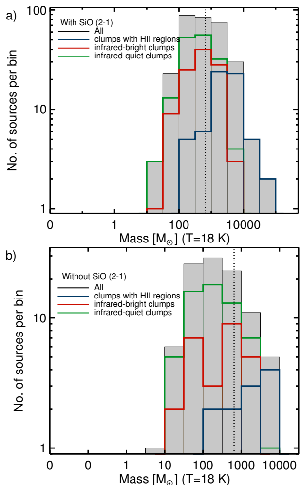
Fig. 8: Histogram of the massive clumps with ( top ) and lacking ( bottom ) SiO (2 – 1) detection from the entire sample and the different categories labelled. The dashed line corresponds to 650 M_{\odot} , which is a crude limit for clumps to form massive stars. Colours are the same as in Fig. 2.
