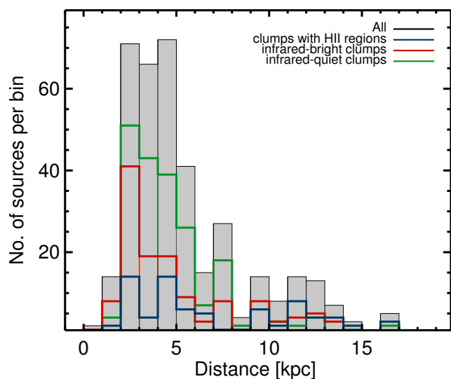
Fig. 2: Distance distribution of the whole sample with the different source types indicated in colours. Black line with grey filling corresponds to the whole sample, blue shows the genuine H II regions, red corresponds to clumps with embedded protostars, and the green histogram shows the infrared-quiet clumps.
