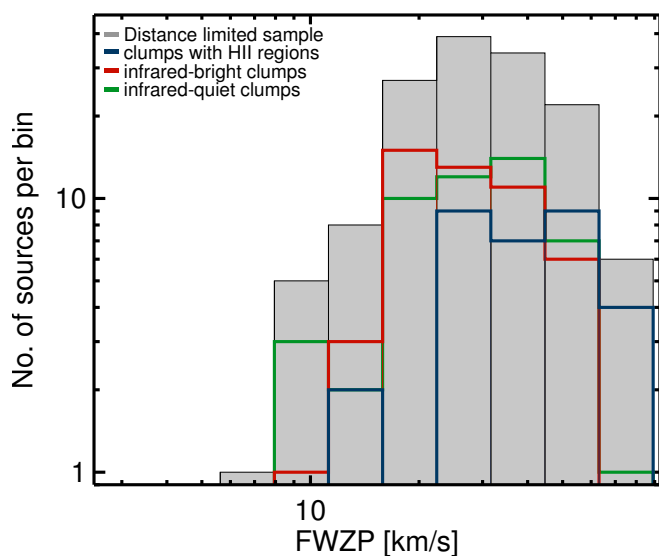
Fig. 10: Histogram of the velocity range for the measured FWZP of the SiO (2–1) emission of the distance-limited subsample (see Sect 3.5). The cutoff in velocity was determined by visual inspection as described in Sect. 4.1, where emission drops to zero.
