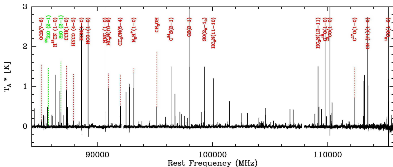
Fig. 1: Complete frequency coverage of the survey carried out with the EMIR instrument at the IRAM 30m telescope towards an example source, showing typical hot-core emission (G29.95–0.02). The SiO 2–1 transition and its isotopologue is labelled in green, other common transitions, which are not used in this paper, are labelled in red.
