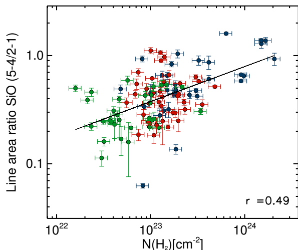
Fig. 18: Same as Fig. 16 for the SiO ( J = 5-4 )/(2–1) ratio. The error is estimated to be 15% for N(H_2) , while for the line ratio the error is calculated from the noise in the two lines: \sigma_{5-4/2-1} = \text{area}_{5-4}/\text{area}_{2-1} \sqrt{(\sigma_{5-4}/\text{area}_{5-4})^2 + (\sigma_{2-1}/\text{area}_{2-1})^2} . Altogether 100 sources are shown on the plot. Sources classified as clumps with embedded H\text{ II} regions are shown in blue, red circles show the infrared-bright clumps, while green corresponds to the infrared-quiet clumps.
